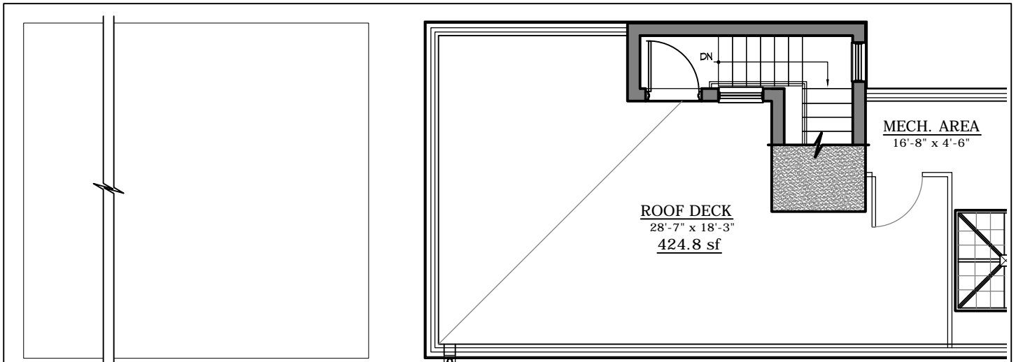
ROOF DECK - 424.8 S.F. TOTAL
