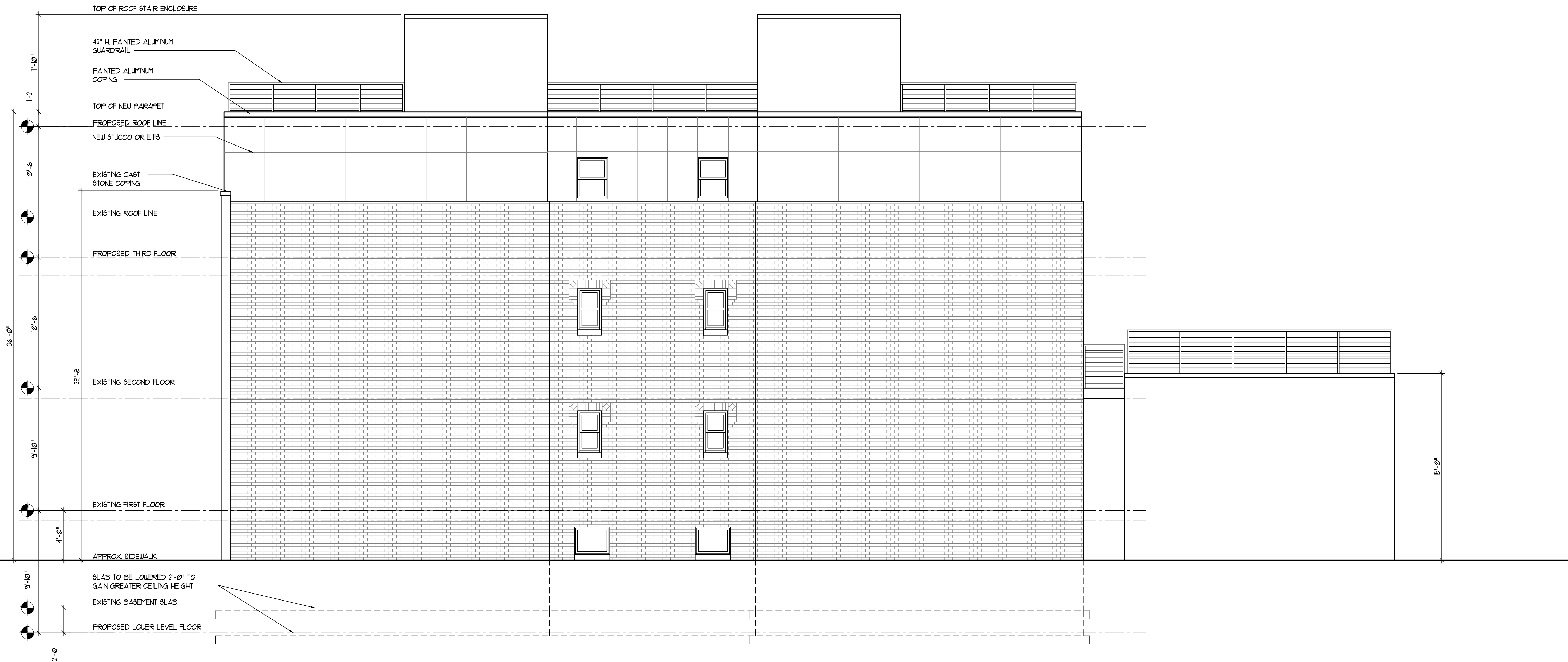
PROPOSED EAST SIDE ELEVATION
